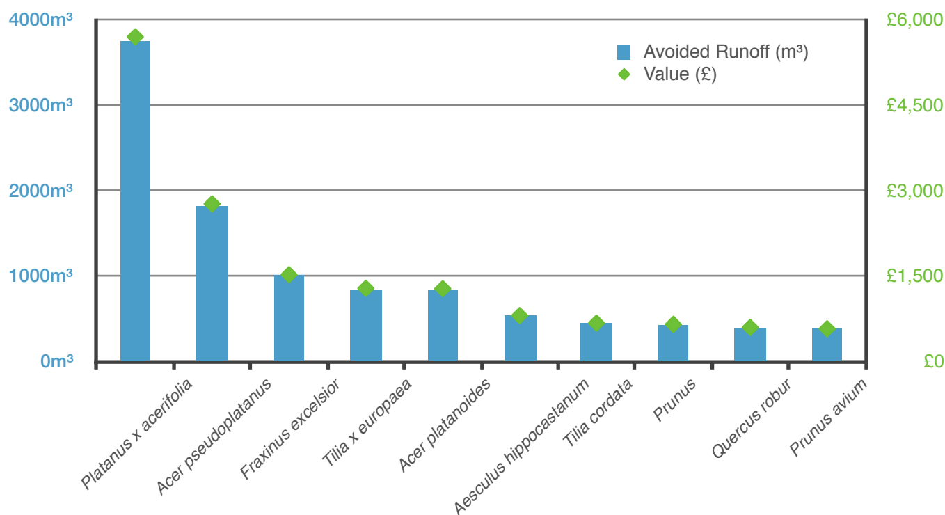
Figure 10: Avoided Runoff by Top Ten Species
