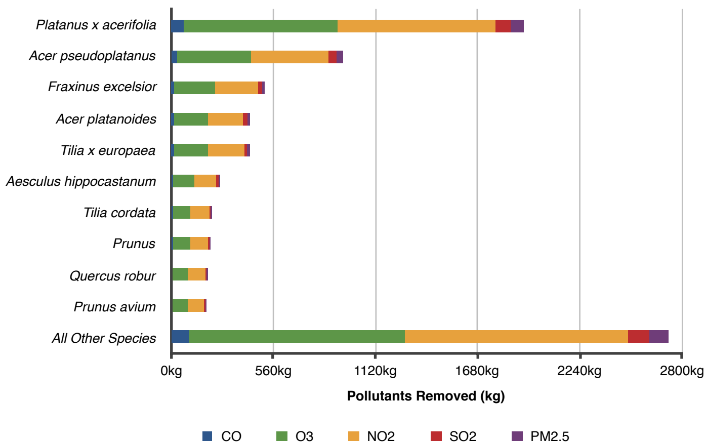
Figure 6: Value of the Pollutants Removed and Quantity Per-Annum within Islington
