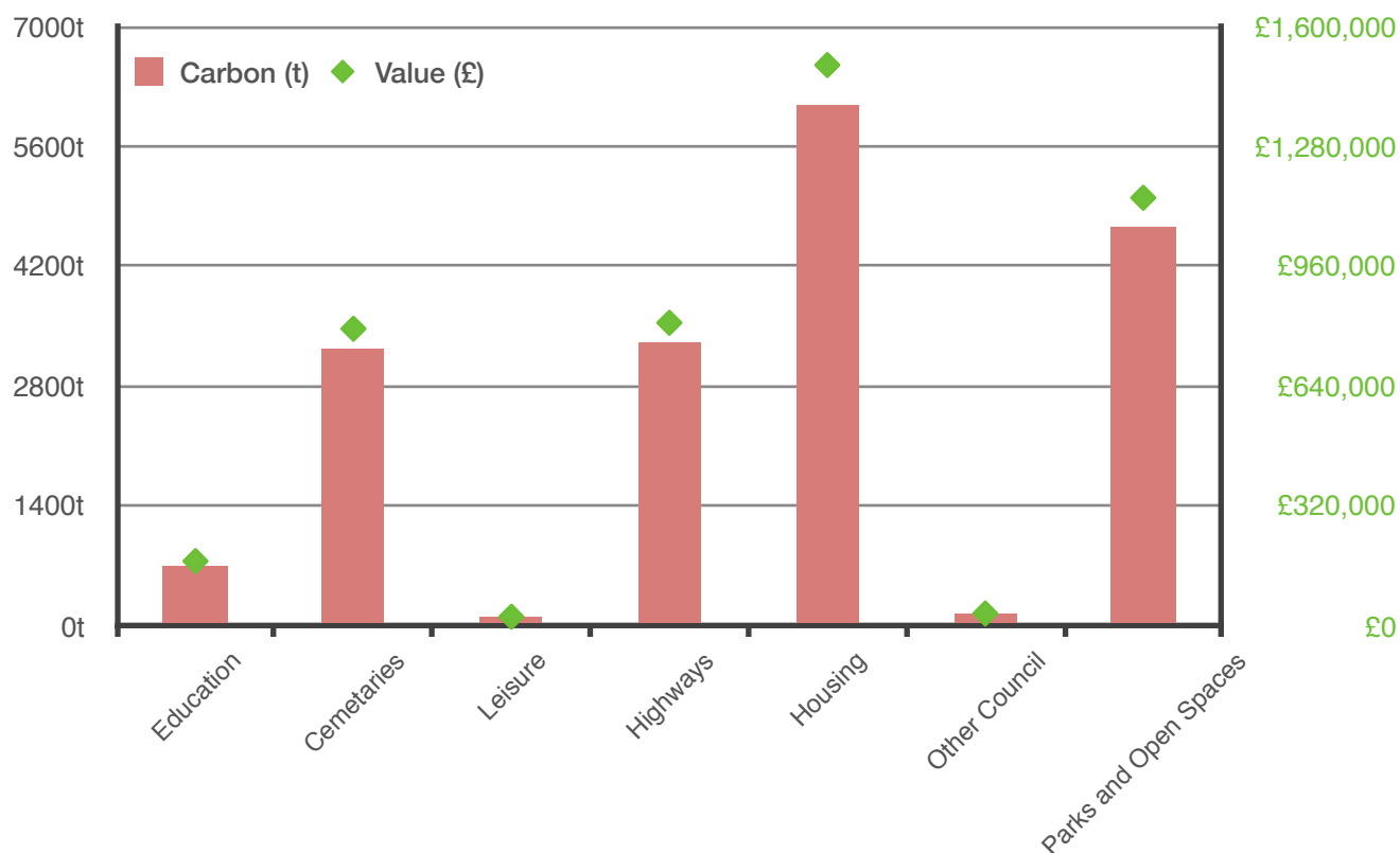
Figure 9: Carbon Stored by Strata
